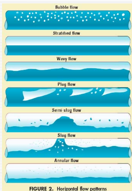
FIGURE 2. Horizontal flow patterns
